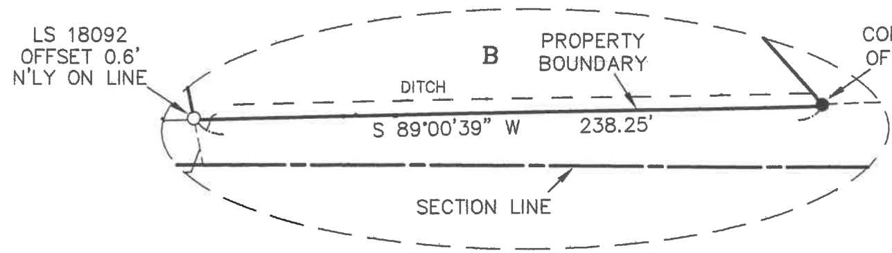
DETAIL NOT TO SCALE
